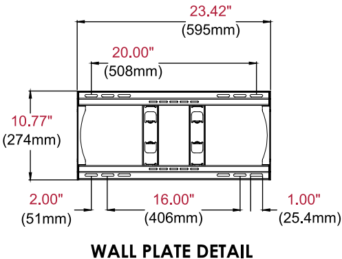
WALL PLATE DETAIL
