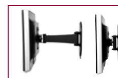
Arm retracts to just 2.50" (64mm) and extends up to 9.61" (244mm) from the wall
