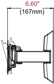
SIDE VIEW EXTENDED +15°/-5° TILT
