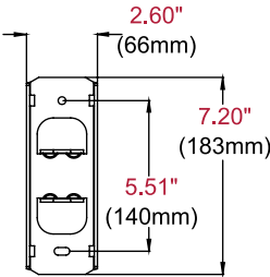
WALL PLATE DETAIL
