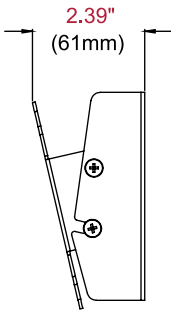
SIDE VIEW +15°/-5° TILT
