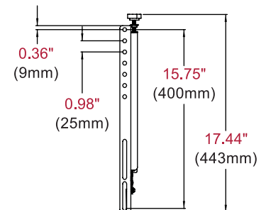
ADAPTOR BRACKET
