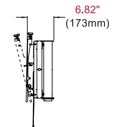
SIDE VIEW 15° TILT
