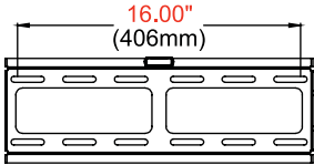
WALL PLATE DETAIL
