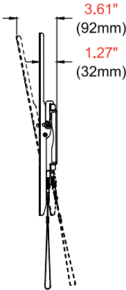
SIDE VIEW +7° TILT
