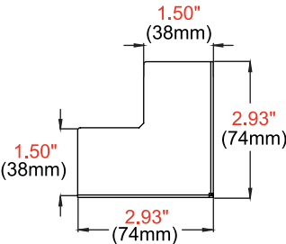
CORNER CAPS
