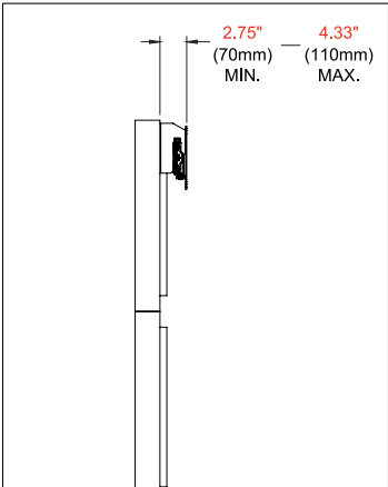
SIDE VIEW WITH dvLED DISPLAY
